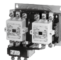
Reversing motor starters SW series
